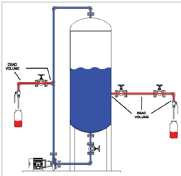
Figure 2 – Sample valve technology and best practices are there to minimize the presence of dead volume.
